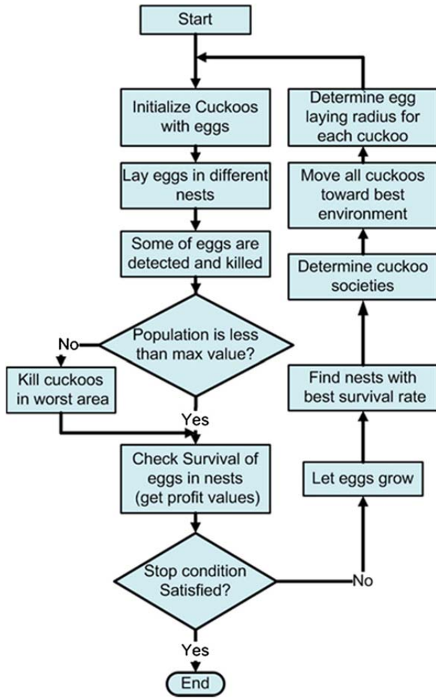
Fig. 1: Flow chart for cuckoo search algorithm
