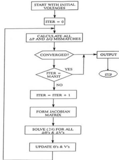
Fig. 2 Flow chart Newton-Raphson Load Flow Analysis
